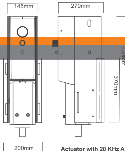
Actuator with 20 KHz Assembly excluding Horn height
